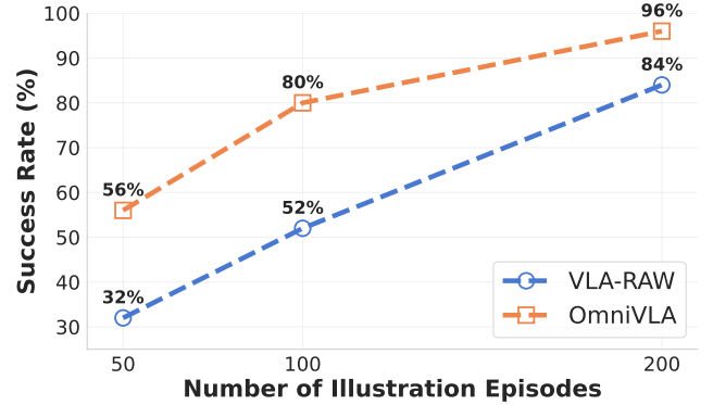
Fig. 6: Success rates over number of demonstration episodes.
