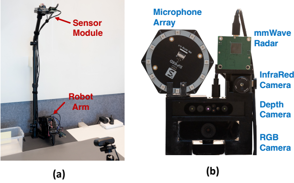
Fig. 4: Hardware Implementation. (a) robot arm and sensor setup (b) sensor module, integrating multiple sensors and cameras.
