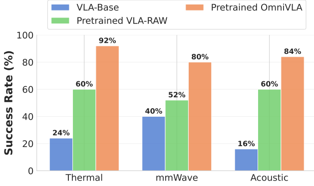
Fig. 7: Success rates when adapting to unseen tasks. We compare the pretrained OmniVLA model with two baselines, VLA-Base: no pretraining, Pretrained VLA-RAW: pretrained with raw sensor images.
